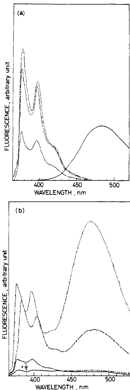
Figure 3. Fluorescence emission spectra of 7.42 \mu\text{M} EP (a) and 13.7 \mu\text{M} DPDL (b) in hexane (— · —), chloroform (· · ·), ethanol (— —), and aqueous buffered solution (pH 5) containing 8% (v/v) ethanol (—) at 20^\circ\text{C} .
