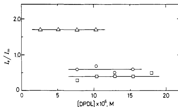
Figure 4. Relative fluorescence quantum efficiencies I_e/I_m for DPDL in ethanol ( \Delta ), chloroform ( \circ ), and hexane ( \square ) as a function of probe concentration.
